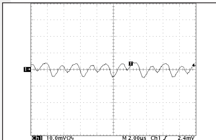
Figure 10: Input terminal current ripple, i_c , at full rated output current and nominal input voltage with SynQor MCOTS filter module. Bandwidth: 20MHz. See Figure 17. Ch 1: i_c (200 mA/div), Time (2μs/div).
